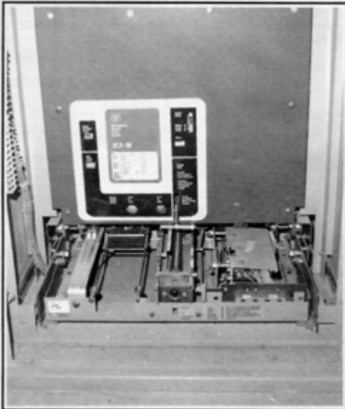
BREAKER RACKED INTO CONNECTED POSITION
