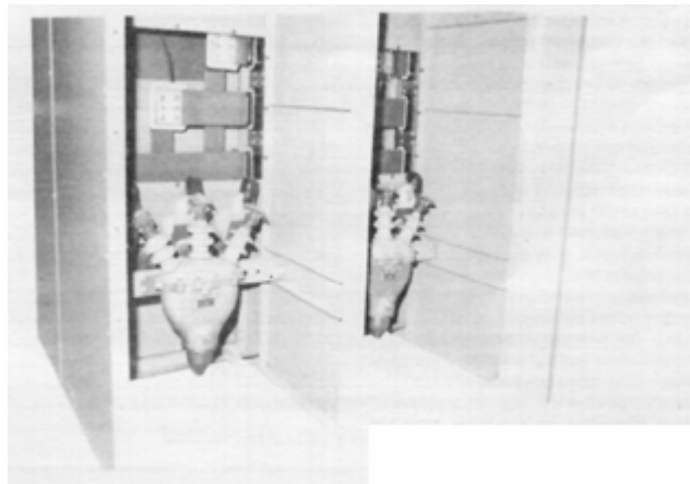
CABLE ENTRY COMPARTMENT WITH MAIN BUS COVERS REMOVED
